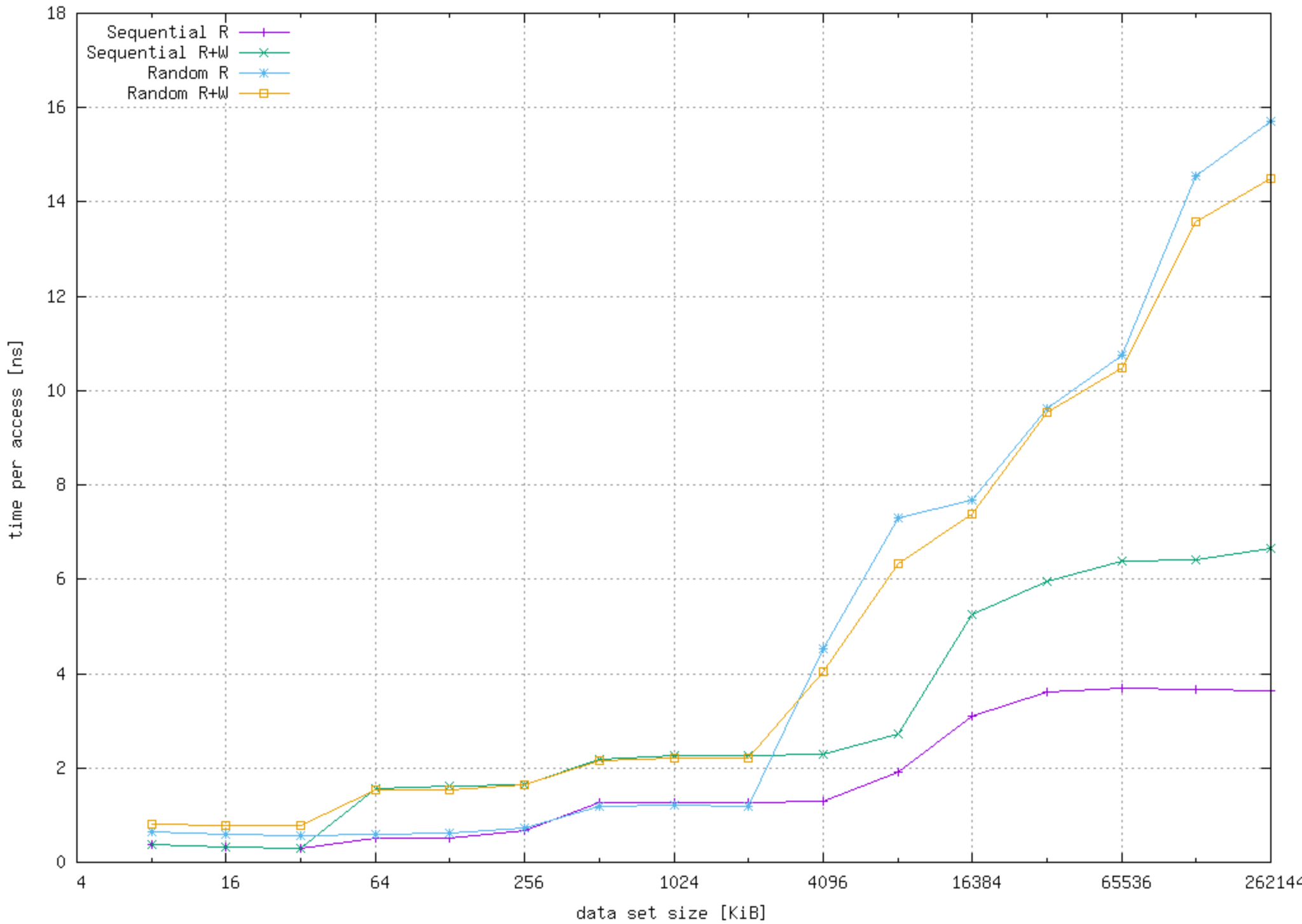
Item size 64 (Array) camelot [Core i7-3770 L1D:32K/8-way L2:256K/8-way L3:8192K/16-way]
